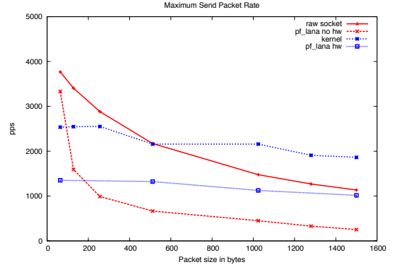
Figure 3: Maximum sending rate comparison.
